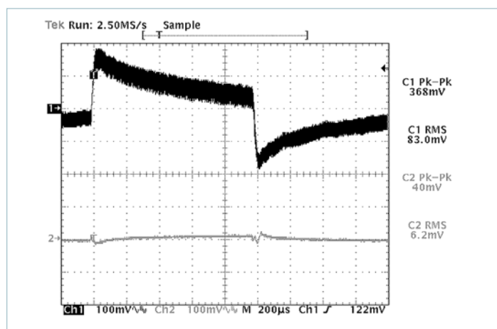
Figure 21 — V375A28C600B and μRAM; Input and output dynamic response C_{TRAN} = 820\mu F Electrolytic; 32.5% of load step of 6.5A (10A – 16.5A); R_{HR} = 178k (Configured as in Figure 7 w/o Trim)
