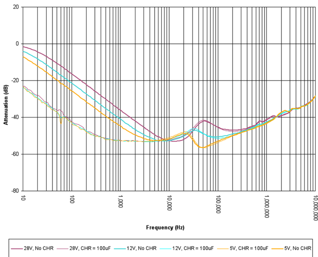
MicroRAM Attenuation: 300mV VHR, 10A Load
