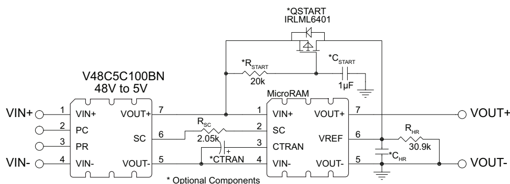
Figure 11 — Typical SC control configuration and an optional start-up circuit. R_{HR} set for 375mV of headroom voltage
