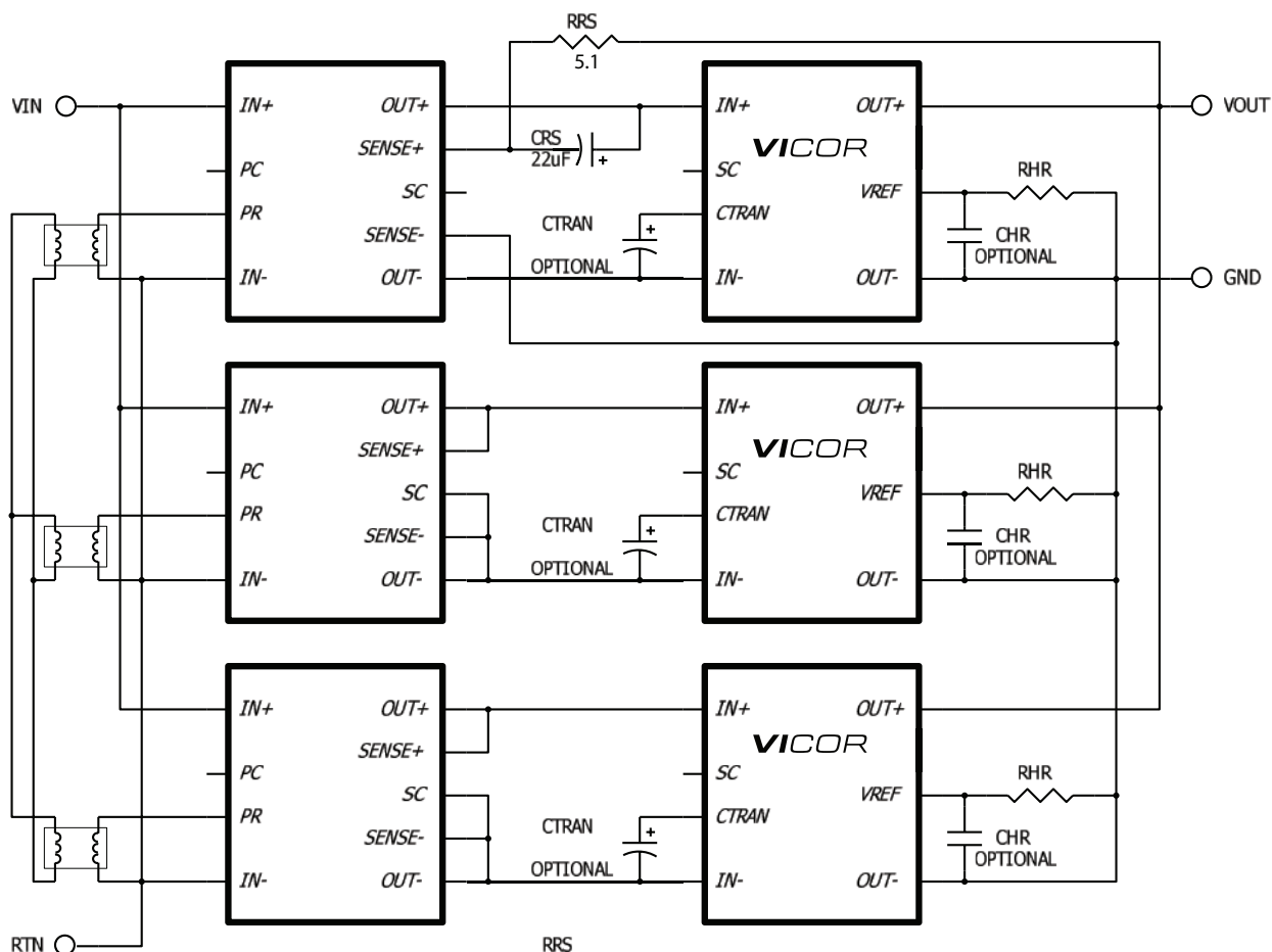
Figure 16 — Recommended paralleling connections of Vicor converters and paired MicroRAMs.
