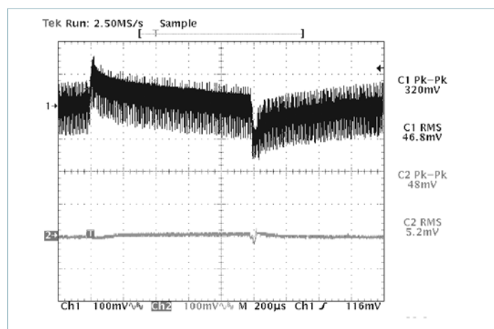
Figure 24 — V300B12C250B and μRAM; Input and output dynamic response C_{TRAN} = 820\mu F Electrolytic; 30% of load step of 6A (10A – 16A); R_{HR} = 80k (Configured as in Figure 8 w/o Trim)
