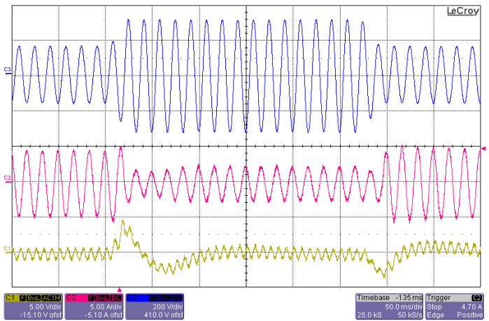
Figure 10: Input voltage transient response with 200µF hold-up capacitor at full load current (115Vrms-230Vrms-115Vrms, 60Hz), Top: Vin (200V/div), Mid: Iin (5A/div), Bottom: Vout (5V/div), Timebase: (50ms/div).
