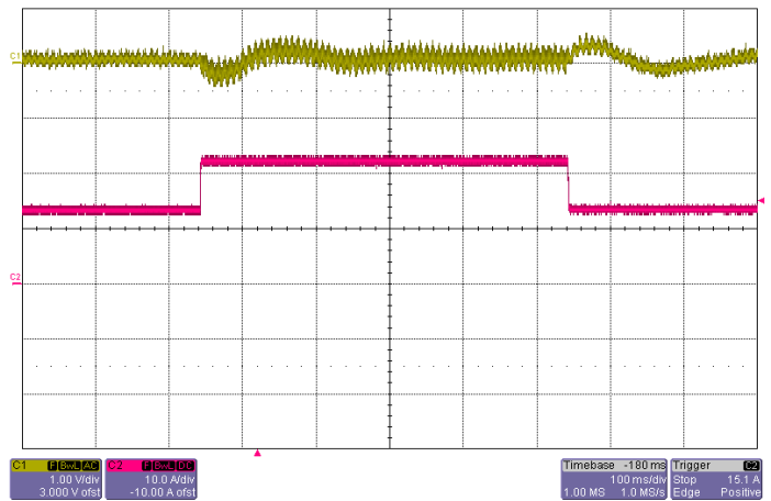
Figure 8: Output voltage response to step-change in load current with 200µF hold-up capacitor (50%-75%-50% of Iout(max), 115Vrms, 60Hz) Top: Vout (1V/div), Bottom: Iout (10A/div), Timebase: (100ms/div).
