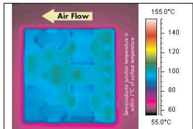
Figure 6: Thermal plot of converter at 40 amp load current with 55°C air flowing at the rate of 200 LFM. Air is flowing from output to input (nominal input voltage).
