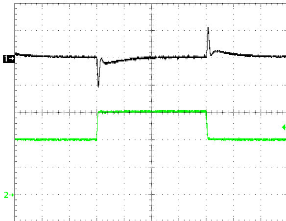
Figure 15: Output voltage response to step-change in load current (50%-75%-50% of Iout(max); dI/dt = 0.1A/μs). Load cap: 10μF, 100 mΩ ESR tantalum cap and 1μF ceramic cap. Ch 1: Vout (200mV/div), Ch 2: Iout (5A/div).
