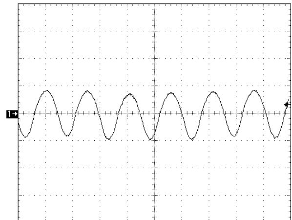
Figure 18: Input Terminal Ripple Current, ic, at full rated output current and nominal input voltage with 10¼H source impedance and 47¼F electrolytic capacitor (200 mA/div). See Figure 17.
