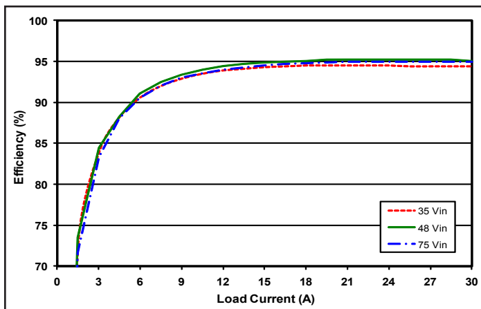
Figure 1: Efficiency at nominal 12V output vs. load current for minimum, nominal, and maximum input voltage at 25°C.
