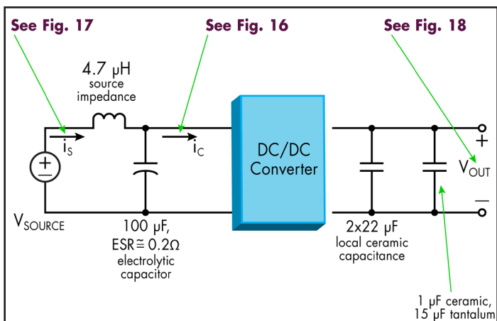
Figure 15: Test set-up diagram showing measurement points for Input Terminal Ripple Current (Fig 16), Input Reflected Ripple Current (Fig 17) and Output Voltage Ripple (Fig 18).
