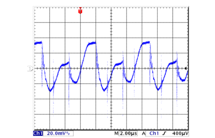
Figure 18: Output voltage ripple at nominal input voltage and rated load current (20mV/div). Load capacitance: 2x22 \mu F ceramic capacitor. Bandwidth: 500 MHz. (Fig 15)
