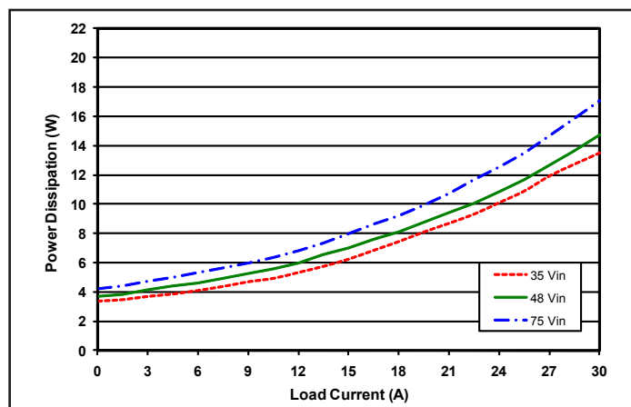
Figure 6: Power dissipation at trimmed-down 6.0V output vs. load current for minimum, nominal, and maximum input voltage at 25°C.
