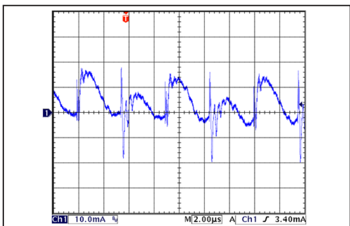
Figure 17: Input reflected ripple current, i_s , through a 4.7 \mu H source inductor at nominal input voltage and rated load current (10mA/div). (Fig 15)
