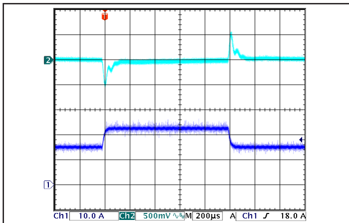
Figure 13: Output voltage response to step-change in load current (50%-75%-50% of I_{out(max)} ; dI/dt = 0.1A/\mu s ). Load cap: 47 \mu F ceramic cap. Top trace: V_{out} (500mV/div), Bottom trace: I_{out} (10A/div).
