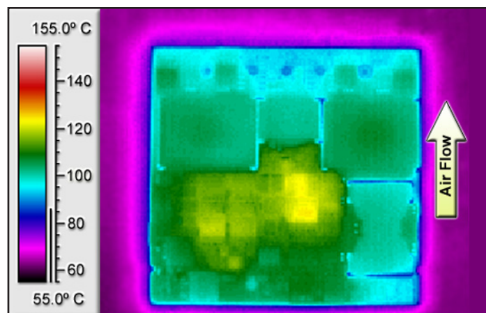
Figure 8: Thermal plot of converter at 25 amp load current (300W) with 55°C air flowing at the rate of 200 LFM. Air is flowing across the converter from input to output (nominal input voltage).
