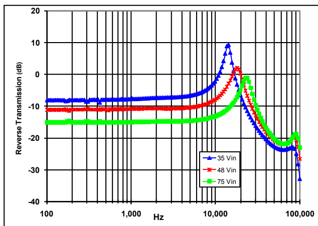
Figure 23: Magnitude of incremental reverse transmission ( RT = i_{in}/i_{out} ) for minimum, nominal, and maximum input voltage at full rated power.
