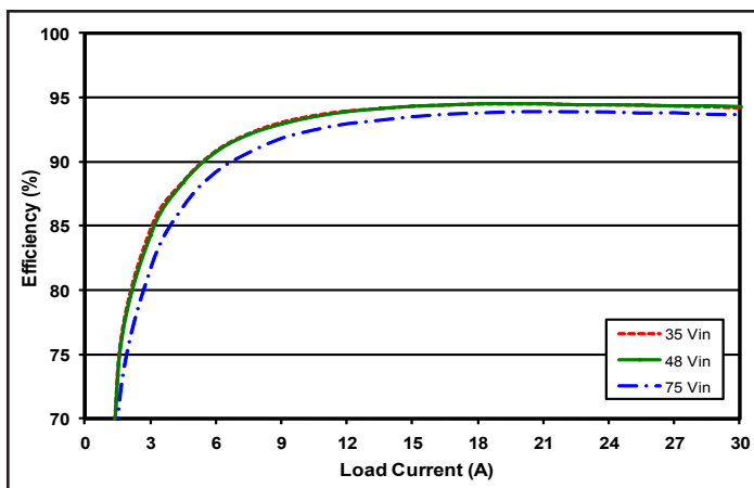
Figure 3: Efficiency at trimmed-down 9.0V output vs. load current for minimum, nominal, and maximum input voltage at 25°C.
