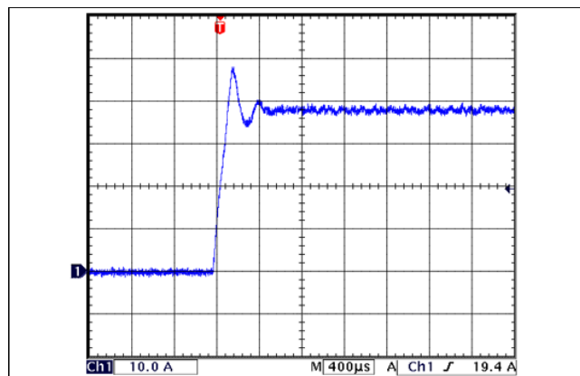
Figure 20: Load current (10A/div) as a function of time when the converter attempts to turn on into a 1mΩ short circuit.
