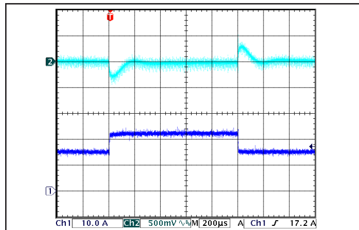
Figure 14: Output voltage response to step-change in load current (50%-75%-50% of I_{out(max)} ; dI/dt = 5A/\mu s ). Load cap: 470 \mu F , 15 m \Omega ESR tantalum cap and 47 \mu F ceramic cap. Top trace: V_{out} (500mV/div), Bottom trace: I_{out} (10A/div).
