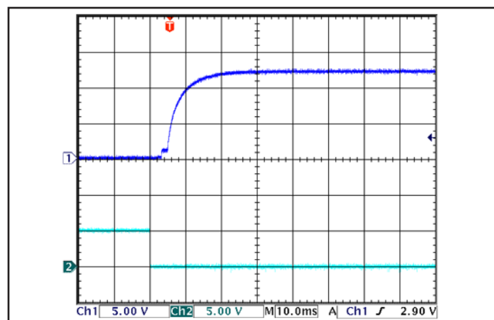
Figure 12: Turn-on transient at zero load (10 ms/div). Top Trace: V out (5V/div). Bottom Trace: ON/OFF input (5V/div).
