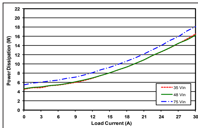
Figure 4: Power dissipation at trimmed-down 9.0V output vs. load current for minimum, nominal, and maximum input voltage at 25°C.
