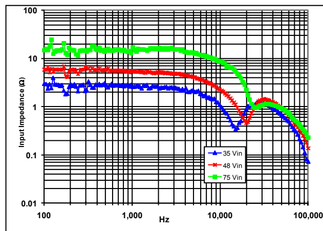
Figure 24: Magnitude of incremental input impedance ( Z_{in} = v_{in}/i_{in} ) for minimum, nominal, and maximum input voltage at full rated power.
