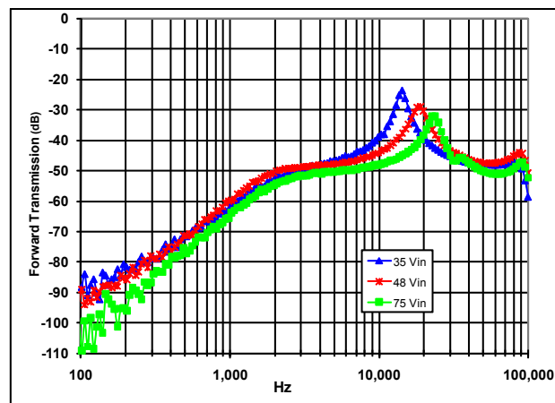
Figure 22: Magnitude of incremental forward transmission ( FT = v_{out}/v_{in} ) for minimum, nominal, and maximum input voltage at full rated power.
