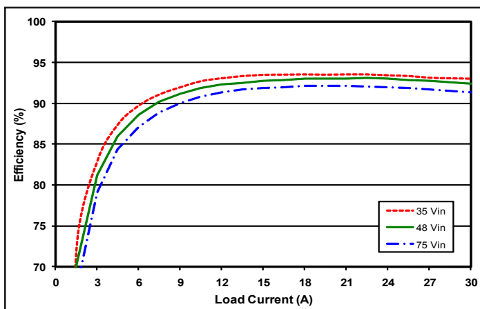
Figure 5: Efficiency at trimmed-down 6.0V output vs. load current for minimum, nominal, and maximum input voltage at 25°C.
