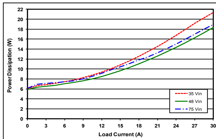
Figure 2: Power dissipation at nominal 12V output vs. load current for minimum, nominal, and maximum input voltage at 25°C.
