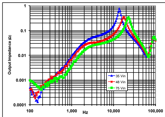
Figure 21: Magnitude of incremental output impedance ( Z_{out} = v_{out}/i_{out} ) for minimum, nominal, and maximum input voltage at full rated power.
