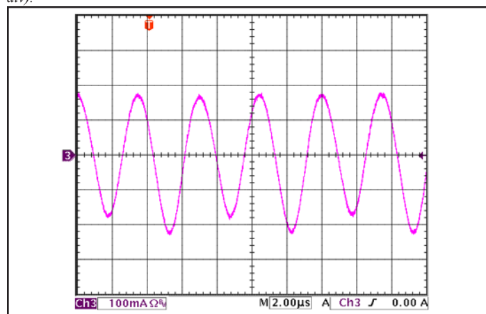
Figure 16: Input terminal ripple current, i_c , at full rated output current and nominal input voltage with 4.7 \mu H source impedance and 100 \mu F electrolytic capacitor (100 mA/div). (Fig 15)
