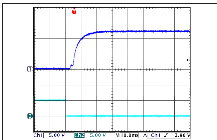
Figure 11: Turn-on transient at full load (resistive load) (10 ms/div). Input voltage pre-applied. Top Trace: V out (5V/div). Bottom Trace: ON/OFF input (5V/div).
