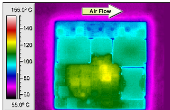
Figure 10: Thermal plot of converter at 24.5 amp load current (294W) with 55°C air flowing at the rate of 200 LFM. Air is flowing across the converter from pin 1 to pin 4 (nominal input voltage).
