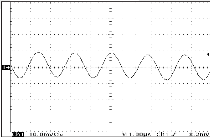
Figure 15: Input reflected ripple current, i_s , through a 10 \mu\text{H} source inductor, using a 1 \mu\text{F} ceramic input capacitor (50 mA/div). See Figure 12.
