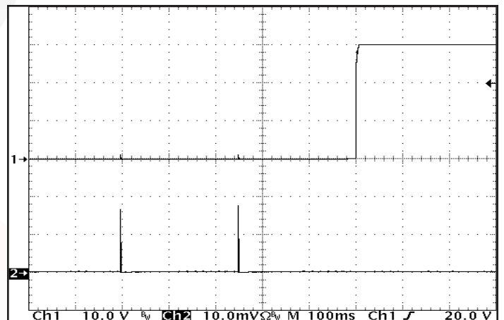
Figure 18: Rise of output voltage after the removal of a short circuit across the output terminals. R_{short} = 5\text{ m}\Omega . Ch1: V_{out} (10 V/div). Ch2: I_{out} (50 A/div). Bandwidth: 20 MHz.
