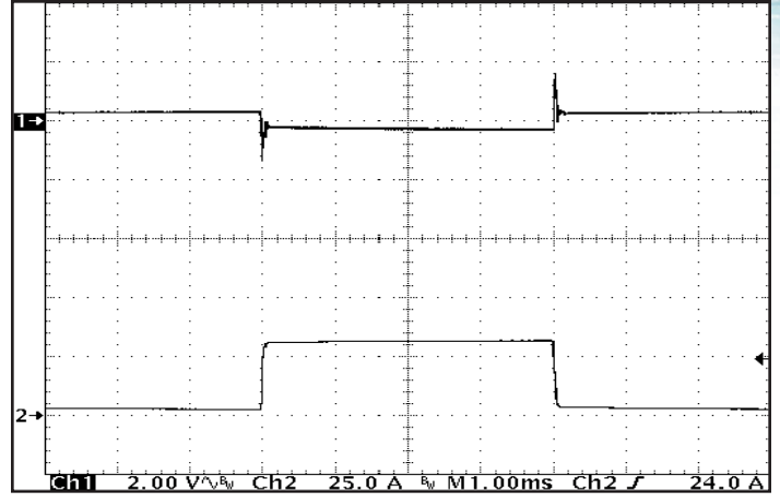
Figure 14: Output voltage response to step-change in load current 10%-100%-10% of I_{out(max)} . Load capacitance: 1 \mu\text{F} ceramic and 10 \mu\text{F} 100 m \Omega ESR tantalum. Ch1: V_{out} (2 V/div). Ch2: I_{out} (25 A/div).
