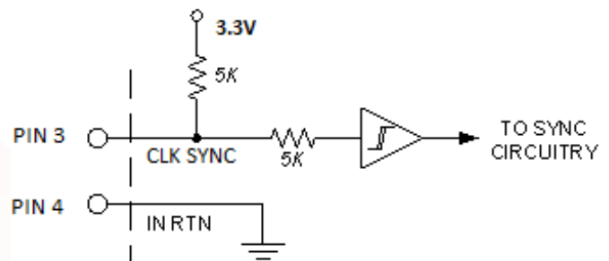
Figure C: Equivalent circuit looking into the CLK SYNC pin with respect to the IN RTN (input return) pin.
