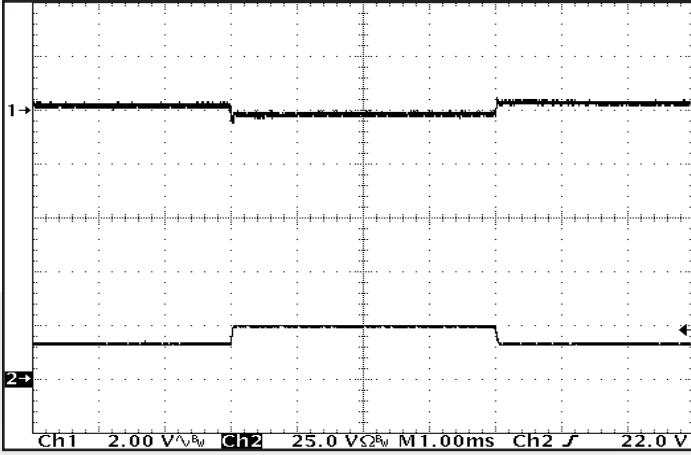
Figure 13: Output voltage response to step-change in load current 50%-75%-50% of I_{out(max)} . Load capacitance: 1 \mu\text{F} ceramic and 10 \mu\text{F} 100 m \Omega ESR tantalum. Ch1: V_{out} (2 V/div). Ch2: I_{out} (25 A/div).
