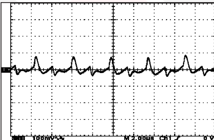
Figure 17: Output voltage ripple, V_{out} , at nominal input voltage and full load (100 mV/div). Bandwidth: 20 MHz. Load capacitance: 1 \mu\text{F} ceramic and 10 \mu\text{F} 100 m \Omega ESR tantalum capacitor. See Figure 12.
