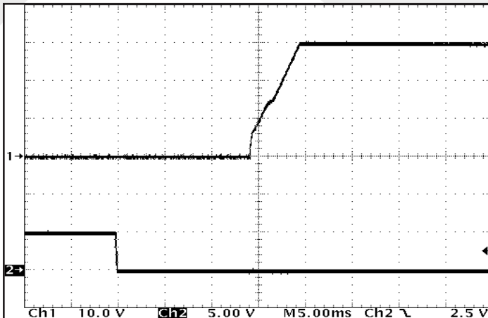
Figure 9: Turn-on transient at half resistive load and 100uF output capacitance initiated by ENA. Input voltage pre-applied. Ch 1: V_{out} (10 V/div). Ch 2: ENA (5 V/div).
