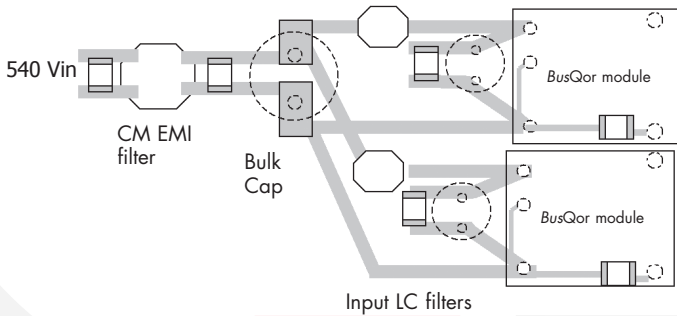
Figure I: Recommended physical implementation of two Bus Qor's in parallel.
