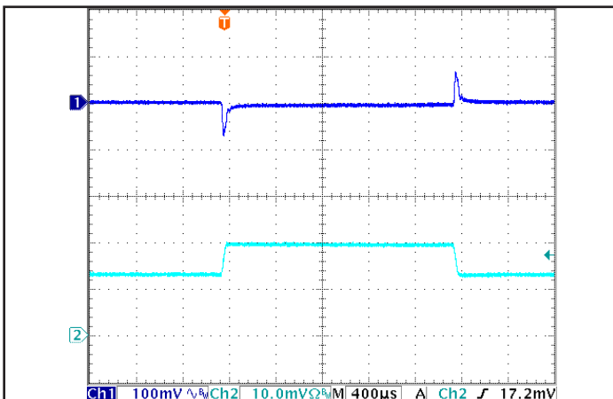
Figure 5: Output voltage response in the SM version unit to step-change in load current (50%-75%-50% of Iout(max); dI/dt = 0.1 A/μs). Load cap: 100 μF electrolytic cap and 1 μF ceramic cap. Ch 1: Vout (100 mV/div), Ch 2: Iout (10 A/div).
