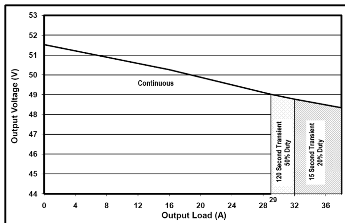
Figure 10: 48 VOUT droop characteristics.
