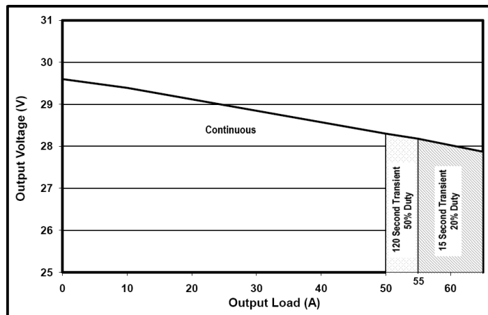
Figure 8: 28 VOUT droop characteristics.
