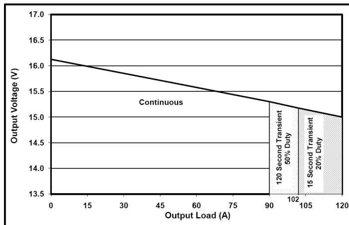
Figure 4: 15 VOUT droop characteristic.
