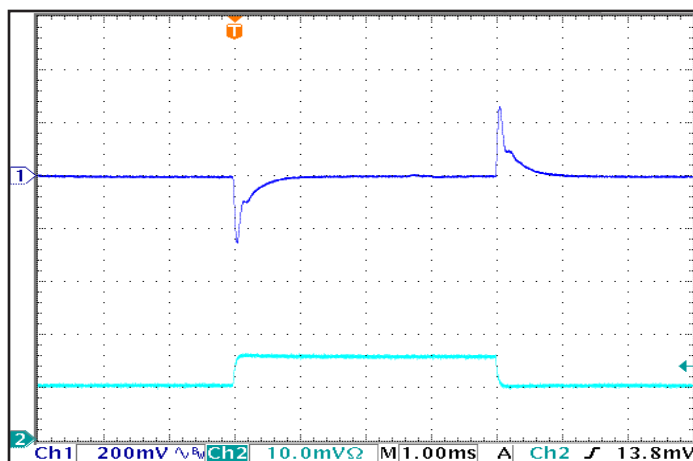
Figure 5: Output voltage response to step-change in load current (50%-75%-50% of Iout(max); dI/dt = 0.1 A/μs). Load cap: 1 μF ceramic capacitor. Ch 1: Vout, Ch 2: Iout(1.0A/div).
